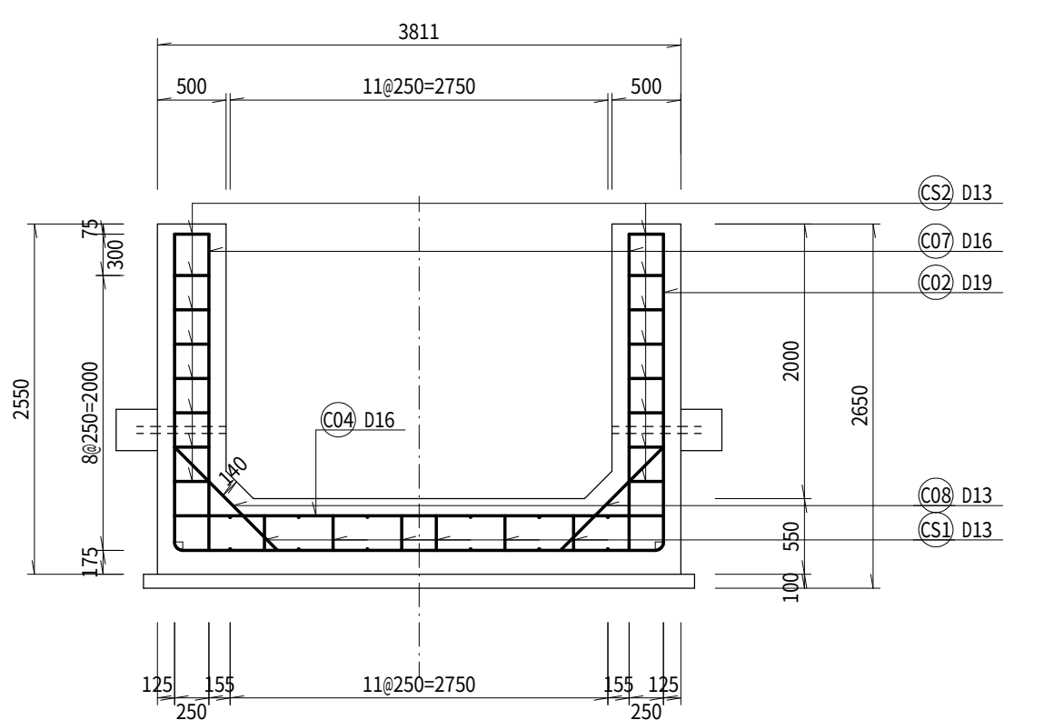
E-E'
